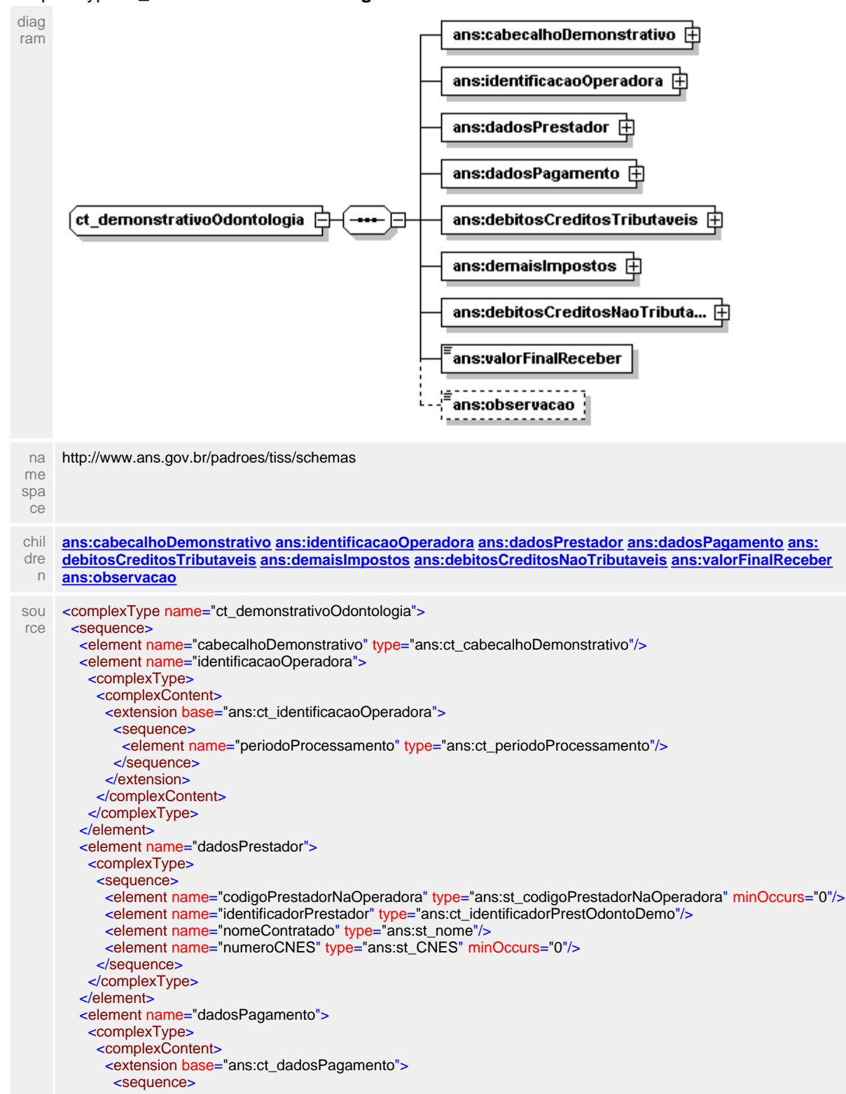
complexType ct_demonstrativoOdontologia
