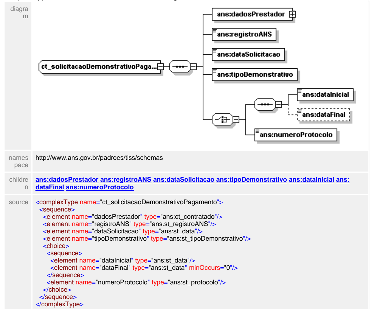
complexType ct_solicitacaoDemonstrativoPagamento
